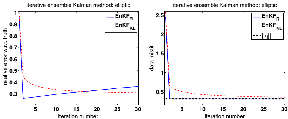
Figure 1. Performance of EnKF R and EnKF KL . Left: relative error with respect to the truth. Right: data misfit.
