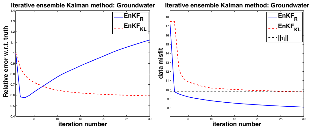
Figure 3. Performance of EnKF R and EnKF KL . Left: relative error with respect to the truth. Right: data misfit.
