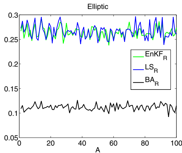
Figure 2. Comparison over different subspaces \mathcal{A} , generated from draws from the prior, of the relative errors of one iteration of EnKF R versus (Tikhonov regularized) least squares (LS R ) and the best approximation (BA R ).
