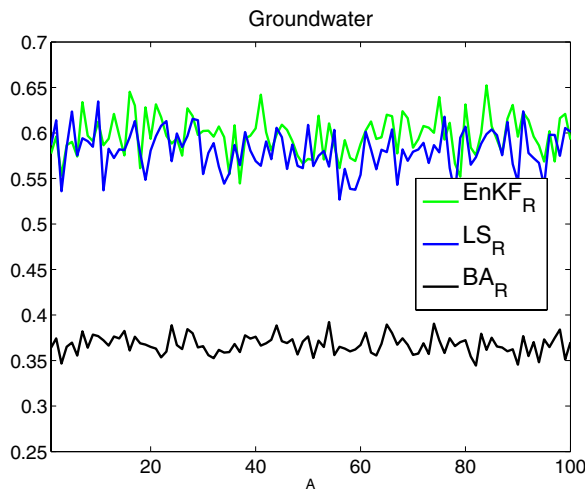
Figure 4. Comparison over different subspaces \mathcal{A} , generated from draws from the prior, of the relative errors of one iteration of EnKF R versus (Newton-CG regularized) least squares (LS R ) and the best approximation (BA R ).
