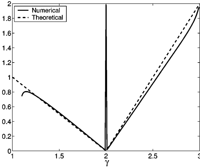
FIG. 4. Convergence rate.
