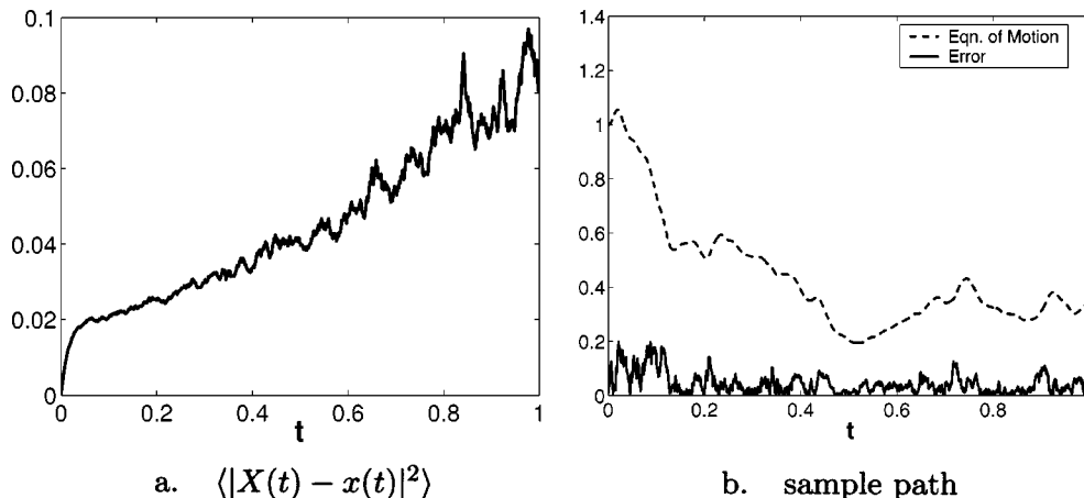
FIG. 2. Difference between the solution of the limiting equation and the equation of motion for \gamma=2 , for \epsilon=0.1 .
