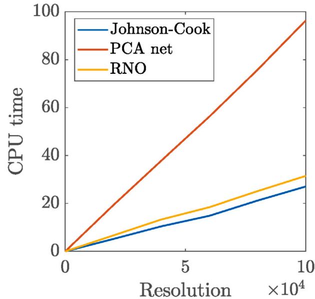
Fig. 13. Computational cost.: CPU time versus number of time steps for the classical Johnson–Cook constitutive law, the PCA-Net proposed in our previous work and the current RNO.
