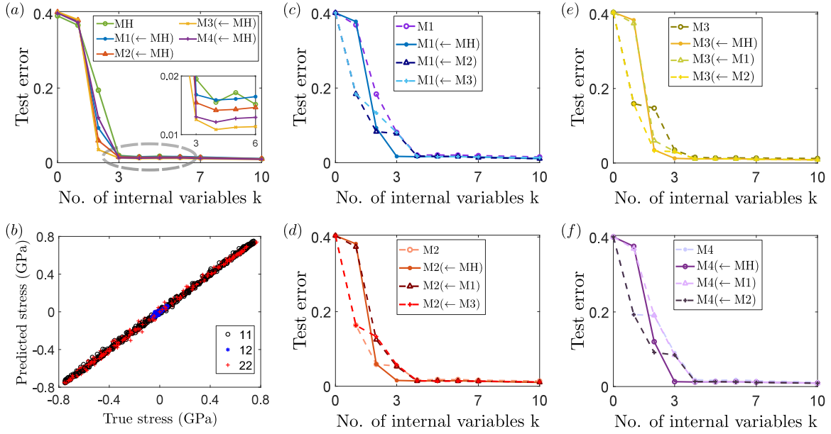
Fig. 3. Approximating an elasto-viscoplastic laminate with no-strain hardening with a recurrent neural operator. (a) Training RNOs with various numbers of internal variables. In each case, we train the homogeneous material (MH) and then use transfer learning. The notation A (\leftarrow B) indicates the case A was trained using transfer learning from B . (b) Comparison of the ground truth and RNO output for eight arbitrarily chosen test strain trajectories for the case M3. (c–f) Training RNOs with various numbers of internal variables both directly and with transfer learning.
