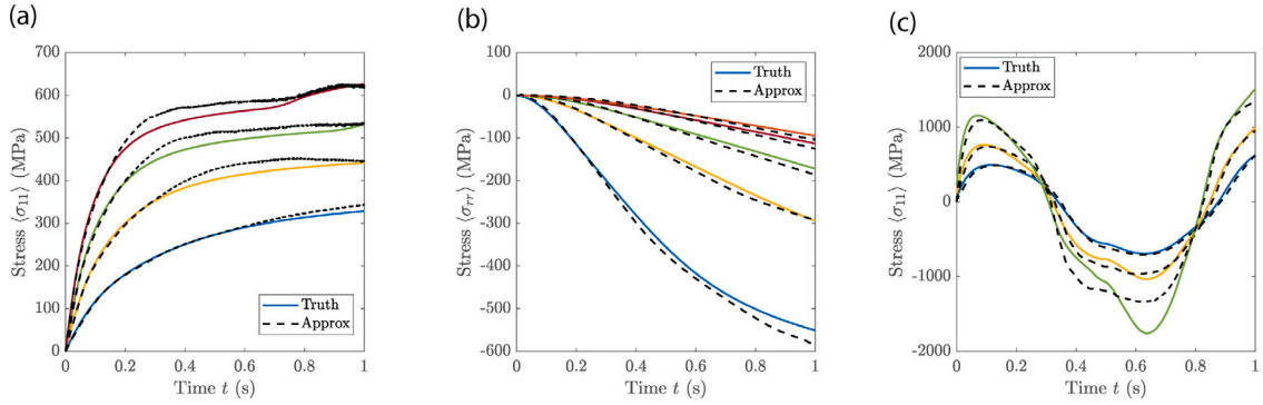
Fig. 9. Testing the trained RNO against classical loading paths. (a) Uniaxial tension. (b) Cavity expansion. (c) cyclic loading.
