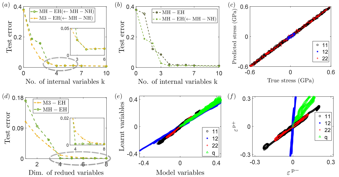
Fig. 6. Approximating an elasto-viscoplastic laminate with exponential strain hardening. (a–c) Learning the strain history to stress history map with a recurrent neural operator: (a) Training RNOs with various numbers of internal variables. In each case, we train the homogeneous material with no hardening (MH-NH) and then use transfer learning. (b) Training RNOs with various numbers of internal variables both directly and with transfer learning. (c) Comparison of the ground truth and RNO output for eight test strain trajectory for the case M3-EH. (d–f) Reducing the number of the internal variables using an auto-encoder: (d) The error of approximating the model variables (state variables in the original laminate model) with an auto encoder for various reduced dimensions. (e) Comparison between the computed values of the model variables and the recovered values from the trained auto-encoder for eight arbitrarily chosen trajectories in the test data for the case M3-EH. (f) The computed values of the model variables in the two layers for eight arbitrarily chosen trajectories in the test data for the case M3-EH.
