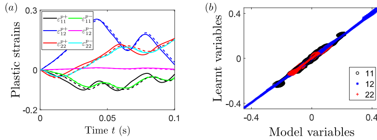
Fig. 5. Reconstructing the micromechanical model variables from the macroscopic internal variables for the case M3. Comparison between the computed values of the model variables and the recovered values from the RNO internal variables for (a) an arbitrarily chosen trajectory and (b) eight arbitrarily chosen trajectories.
