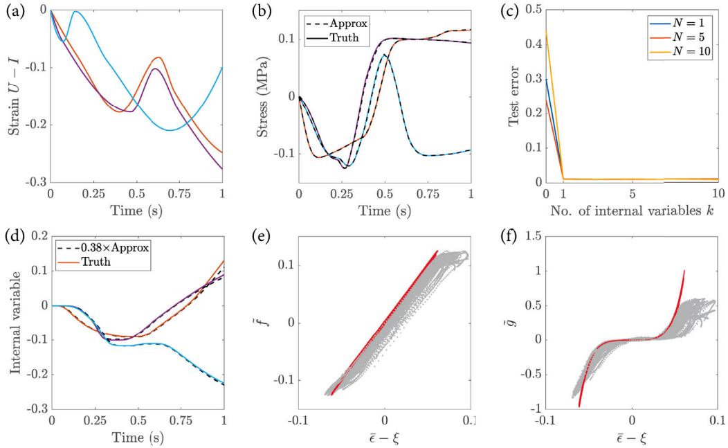
Fig. 1. Approximating elasto-viscoplasticity in one dimension with a recurrent neural operator. (a) Three typical inputs used to train and test the RNO. (b) Comparison of the result of the unit cell problem of a three-phase material ( N = 3 ) corresponding to the inputs in (a) (“Truth”) with the output of the trained RNO with one internal variable ( k = 1 ) with the same input (“Approx”). (c) The average test error for varying number of internal variables, and for varying number of constituents. (d) A comparison of the learnt and actual internal variable for a typical instance of test data in the case of a homogenous material. (e) Comparison of the actual and learnt function \tilde{f} . (f) Comparison of the actual and learnt function \tilde{g} .
