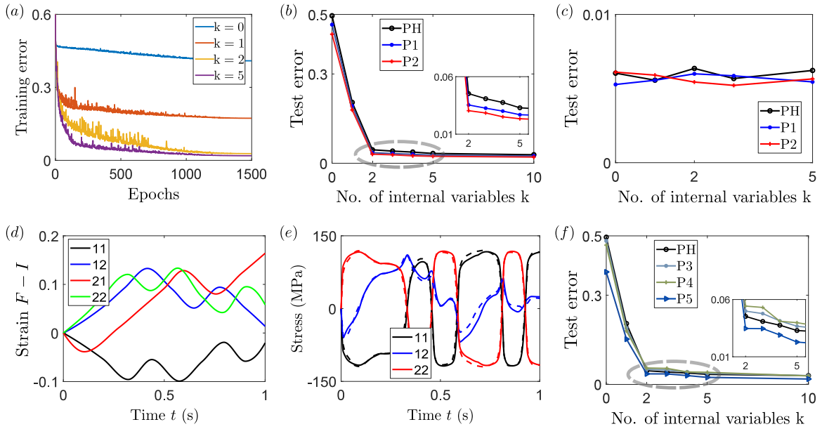
Fig. 7. Approximating two dimensional polycrystalline elasto-viscoplasticity with a recurrent neural operator. (a) Training RNOs with various numbers of internal variables. (b) Test error of the trained RNOs of the deviatoric stress with various number of internal variables and rate hardening cases. (c) Test error of the trained RNOs of the hydrostatic pressure with various number of internal variables and rate hardening cases. (d) A typical average deformation gradient history input test data. (e) Comparison of the resulting deviatoric stress history for the test data (solid) and the prediction of the RNO with two internal variables (dashed). (f) Test error of the trained RNOs of the deviatoric stress with various number of internal variables and strain hardening cases.
