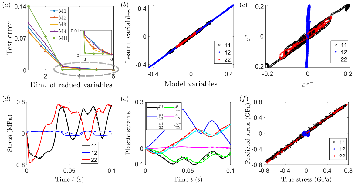
Fig. 4. Reducing the number of the model variables using an auto-encoder. (a) The error of approximating the model variables (state variables in the original laminate model) with an auto encoder for various reduced dimensions. (b) Comparison between the computed values of the model variables and the recovered values from the trained auto-encoder for eight arbitrarily chosen trajectories in the test data for the case M3. (c) The computed values of the model variables in the two layers for eight arbitrarily chosen trajectories in the test data for the case M3. (d) Comparison of the computed stress response (solid) with the learnt stress response (dashed) for a typical test trajectory for the case M3. (e) Comparison of the computed plastic strains model variables (solid) with the reconstructed plastic strain (dashed) for a typical test trajectory for the case M3. (f) Comparison of the computed stress with the learnt stress for eight test trajectories for the case M3.
