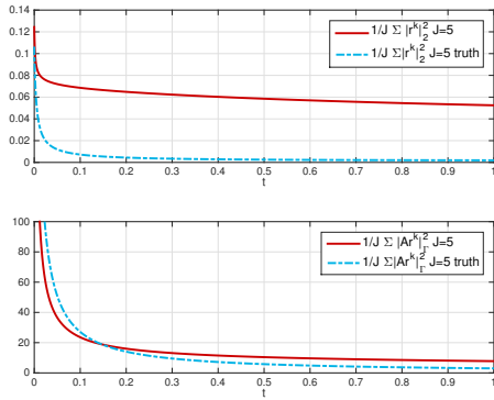
FIG. 11. Quantities |r|_2^2 , |Ar|_\Gamma^2 w.r. to time t , J = 5 based on KL expansion of C_0 = \beta(A - id)^{-1} (red), J = 5 minimizing the contribution of Ar_\perp^{(j)}(t) (blue), \beta = 10 , K = 2^4 - 1 , \eta \sim \mathcal{N}(0, 0.01^2 id) , Bayesian stopping rule.
