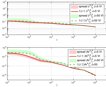
FIG. 20. Quantities |r|_2^2, |Ar|_\Gamma^2 w.r. to time t , J = 5 with variance inflation (red) and J = 50 with variance inflation (green), \beta = 10 , K = 2^4 - 1 , initial ensemble chosen based on KL expansion of C_0 = \beta(A - id)^{-1} .
