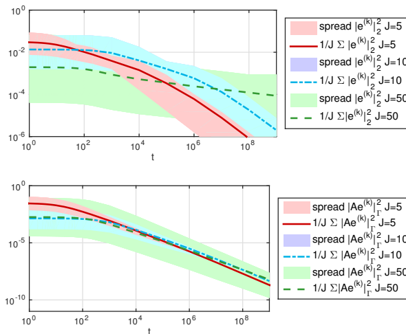
FIG. 1. Quantities |e|_2^2, |Ae|_\Gamma^2 with respect (w.r.) to time t, J = 5 (red), J = 10 (blue), and J = 50 (green), \beta = 10, K = 2^4 - 1 , initial ensemble chosen based on KL expansion of C_0 = \beta(A - id)^{-1} .
