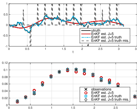
FIG. 16. Comparison of the EnKF estimate with the truth and the observations, J = 5 based on KL expansion of C_0 = \beta(A - id)^{-1} (red), J = 5 adaptively chosen (blue), J = 5 minimizing the contribution of \varphi_{\perp} w.r. to misfit (gray), \beta = 10 , K = 2^4 - 1 , \eta \sim \mathcal{N}(0, 0.001^2 id) .
