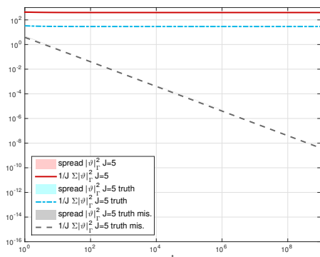
FIG. 15. Misfit |\varphi|_{\Gamma}^2 w.r. to time t , J = 5 based on KL expansion of C_0 = \beta(A - id)^{-1} (red), J = 5 adaptively chosen (blue), J = 5 minimizing the contribution of \varphi_{\perp} w.r. to misfit (gray), \beta = 10 , K = 2^4 - 1 , \eta \sim \mathcal{N}(0, 0.001^2 id) .
