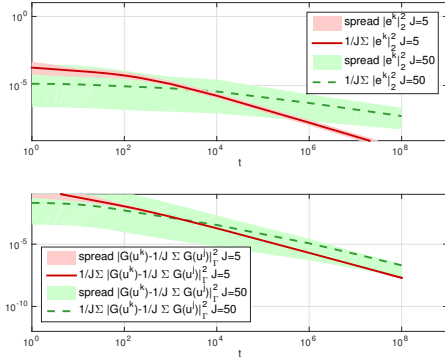
FIG. 17. Quantities |e^{(k)}|_2^2 , |\mathcal{G}(u^{(k)}) - \frac{1}{J} \sum_{j=1}^J \mathcal{G}(u^{(j)})|_2^2 w.r. to time t , J = 5 (red) and J = 50 (green), initial ensemble chosen based on KL expansion of C_0 = (-\Delta)^{-2} .
