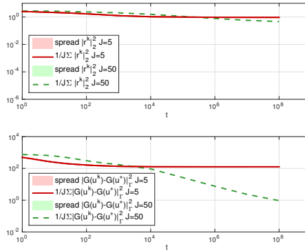
FIG. 18. Quantities |r^{(k)}|_2^2 , |\mathcal{G}(u^{(k)}) - \mathcal{G}(u^\dagger)|_2^2 w.r. to time t , J = 5 (red) and J = 50 (green), initial ensemble chosen based on KL expansion of C_0 = (-\Delta)^{-2} .
