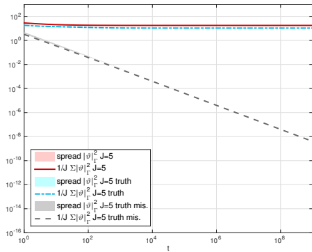
FIG. 13. Misfit |\theta|_\Gamma^2 w.r. to time t , J = 5 based on KL expansion of C_0 = \beta(A - id)^{-1} (red), J = 5 adaptively chosen (blue), J = 5 minimizing the contribution of \theta_\perp w.r. to misfit (gray), \beta = 10 , K = 2^4 - 1 , \eta \sim \mathcal{N}(0, 0.01^2 id) .
