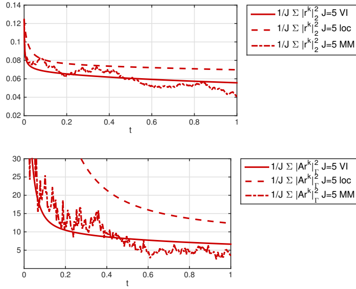
FIG. 26. Quantities |r|_2^2, |Ar|_\Gamma^2 w.r. to time t , J = 5 (red) for the discussed variants, \beta = 10 , \beta = 10 , K = 2^4 - 1 , initial ensemble chosen based on KL expansion of C_0 = \beta(A - id)^{-1} .
